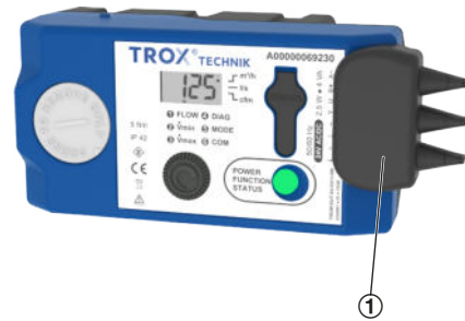
Compact controller XM0-J6 for TVE and TVE-Q (with attached terminal cover)
